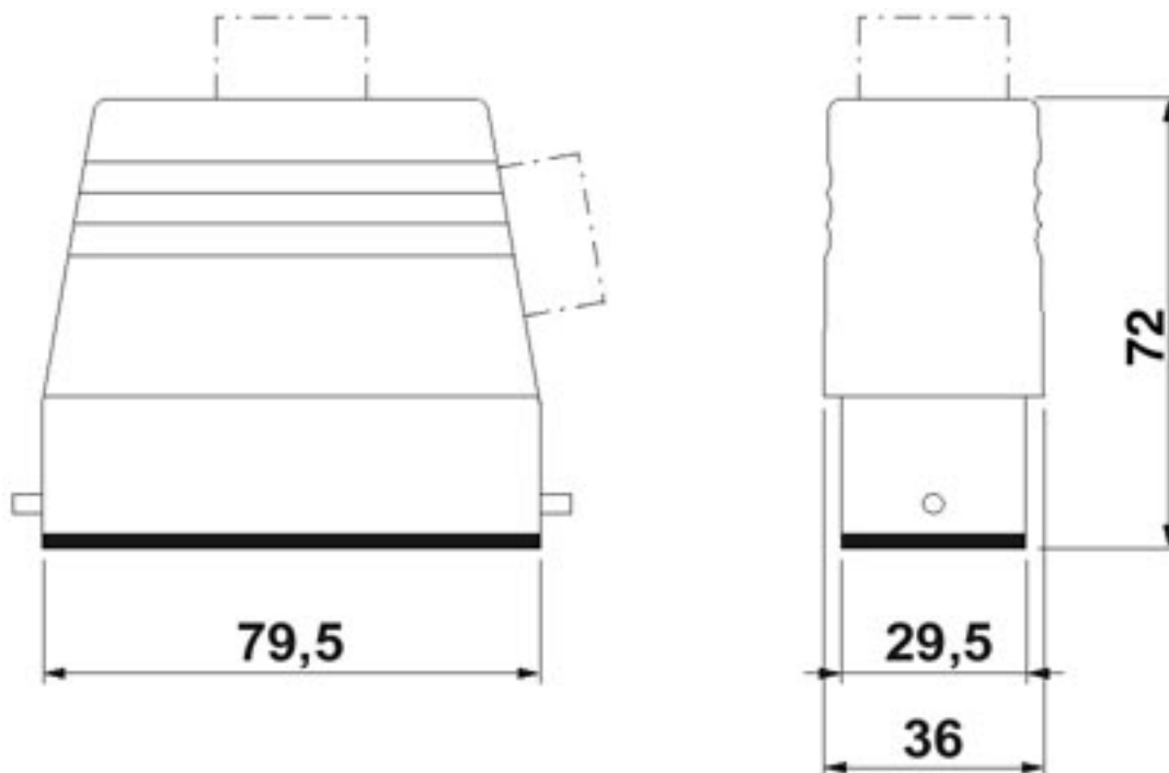
Dimensioned drawing
