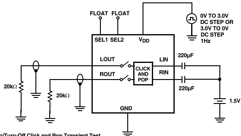
FIGURE 6. CLICK AND POP TEST CIRCUIT #2
