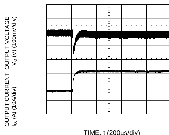
Figure 30. Transient Response to Dynamic Load Change from 25% to 50 % of full load current.
