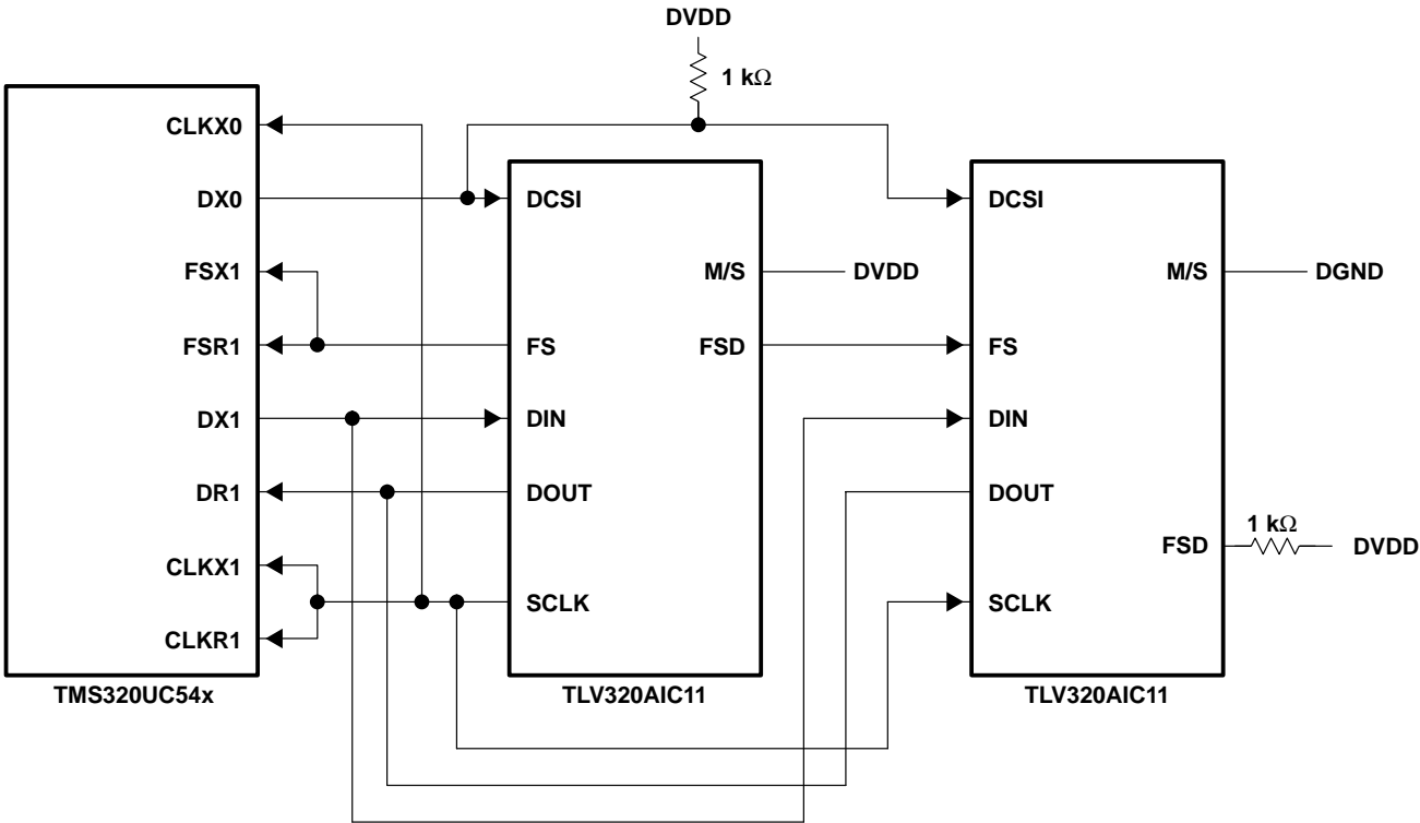
Figure 3–8. Direct Configuration
