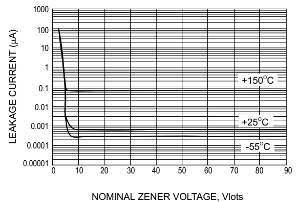
TYPICAL LEAKGE CURRENT
