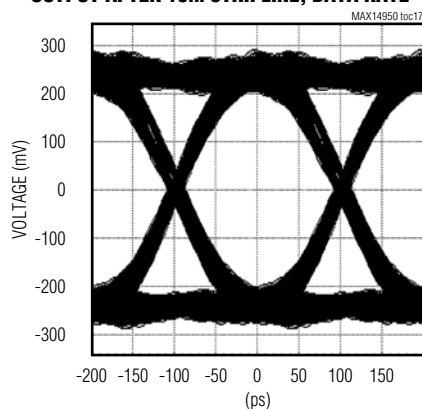
INEQ0 = INEQ1 = 0, V_{IN} = 200\text{mVp-p} , OEQ2 = 0, OEQ1 = 1, OEQ0 = 1, OUTPUT AFTER 19in STRIPLINE, DATA RATE = 56T/s
