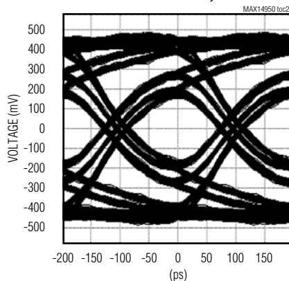
INEQ0 = INEQ1 = 0, V_{IN} = 200\text{mV}_{p-p} , OEQ2 = 0, OEQ1 = 0, OEQ0 = 1, DATA RATE = 8GT/s
