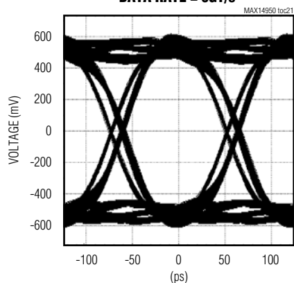
INEQ0 = INEQ1 = 0, V_{IN} = 200\text{mV}_{p-p} , OEQ2 = 0, OEQ1 = 1, OEQ0 = 0, DATA RATE = 8GT/s
