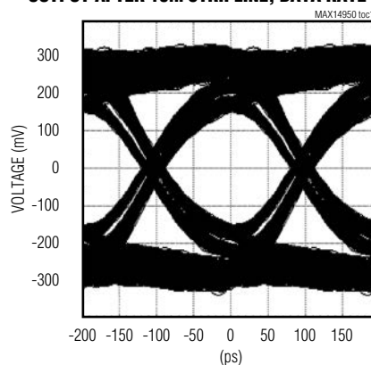
INEQ0 = INEQ1 = 0, V_{IN} = 200\text{mVp-p} , OEQ2 = 1, OEQ1 = 0, OEQ0 = 1, OUTPUT AFTER 19in STRIPLINE, DATA RATE = 56T/s
