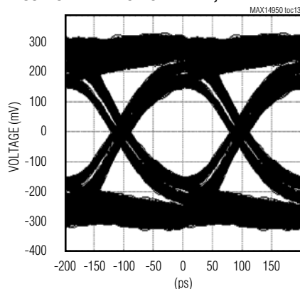
INEQ0 = INEQ1 = 0, V_{IN} = 200\text{mVp-p} , OEQ2 = 1, OEQ1 = 1, OEQ0 = 0, OUTPUT AFTER 19in STRIPLINE, DATA RATE = 56T/s
