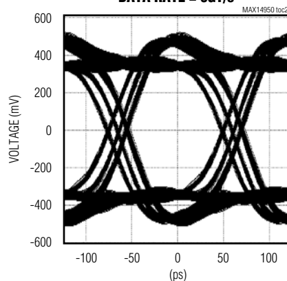
INEQ0 = INEQ1 = 0, V_{IN} = 200\text{mV}_{p-p} , OEQ2 = 0, OEQ1 = 1, OEQ0 = 1, DATA RATE = 8GT/s
