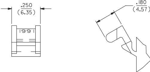
DETAIL I PREBENT MOUNTING EAR (SCALE 4:1)
