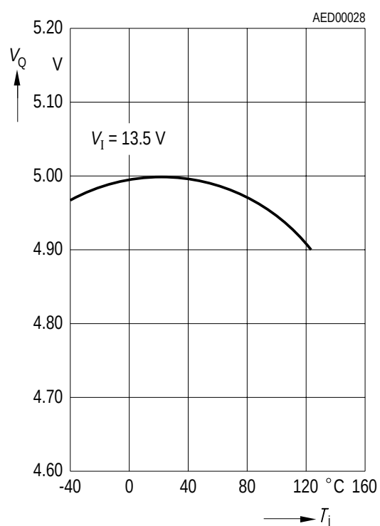
Output Voltage versus Temperature
