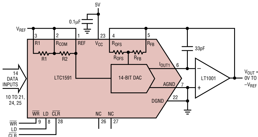
Figure 1a. Unipolar Operation (2-Quadrant Multiplication) V_{OUT} = 0\text{V} to -V_{REF}
