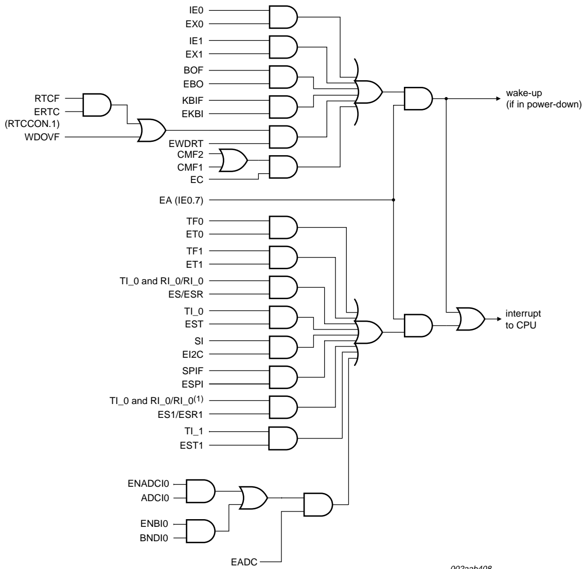
Fig 6. Interrupt sources, interrupt enables, and power-down wake-up sources
