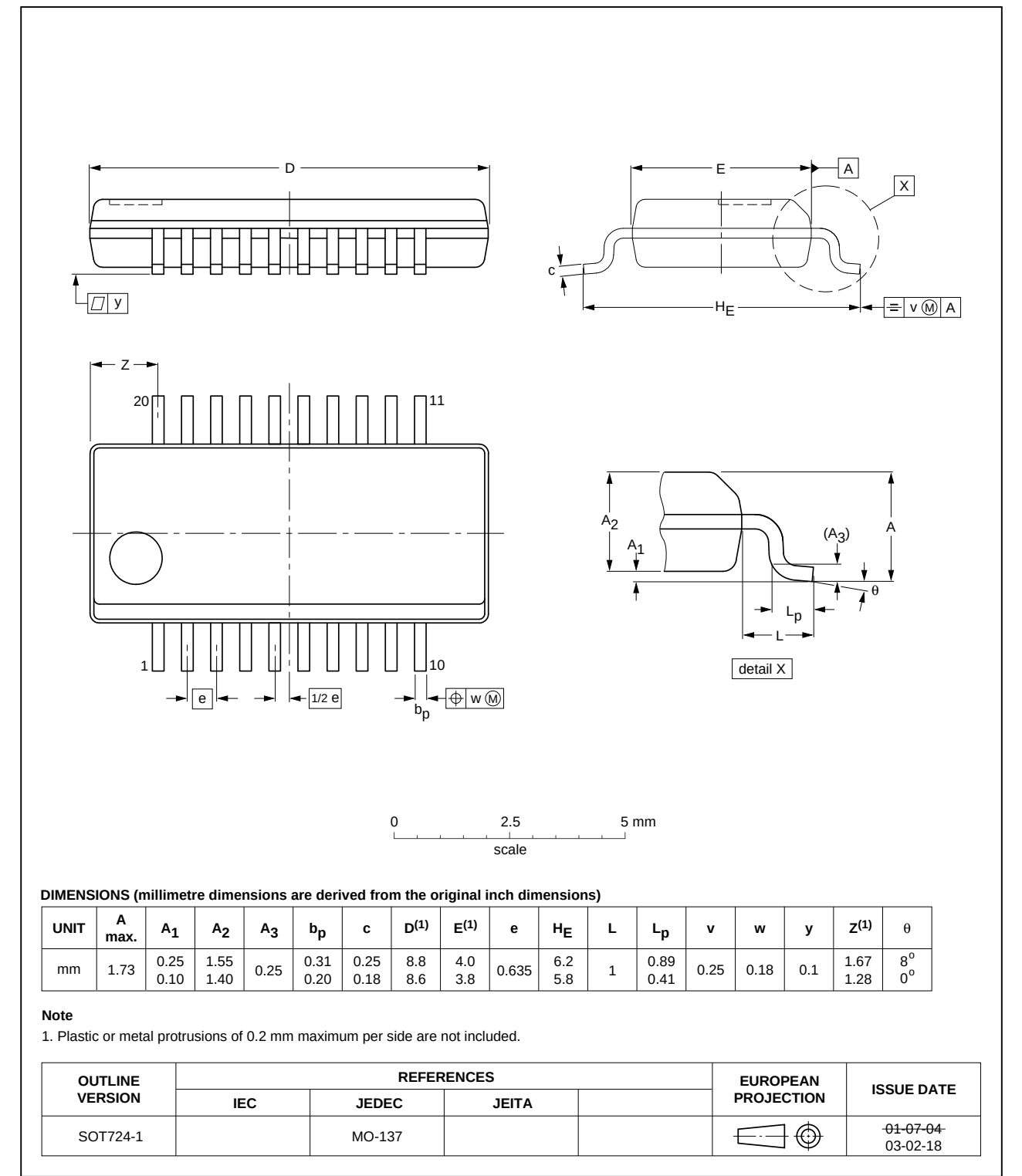
Fig 10. Package outline SOT724-1 (SSOP20)
