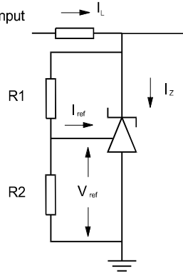
Fig 2 – Test Circuit for V_z > V_{ref}
