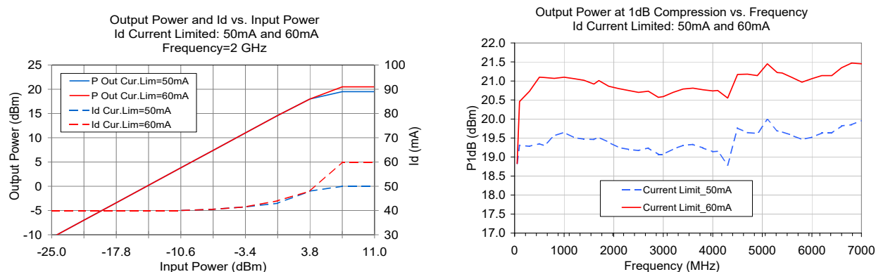
Fig 2. Output Power and I_d vs. Input Power and Frequency. Performance measured on Mini-Circuits Characterization test board TB-502+. See Characterization Test Circuit (Fig. 1) Measurements performed with current ( I_d ) limited as noted.
