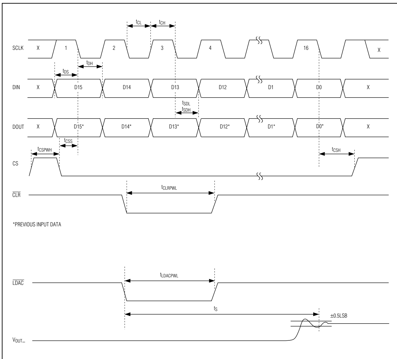
Figure 4. Timing Diagram
