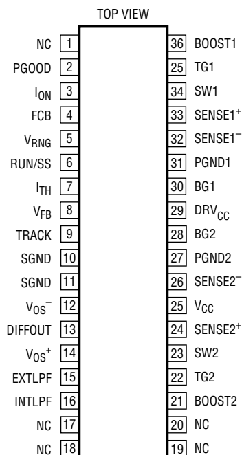
G PACKAGE 36-LEAD PLASTIC SSOP T_{JMAX} = 125^{\circ}C , \theta_{JA} = 95^{\circ}C/W
