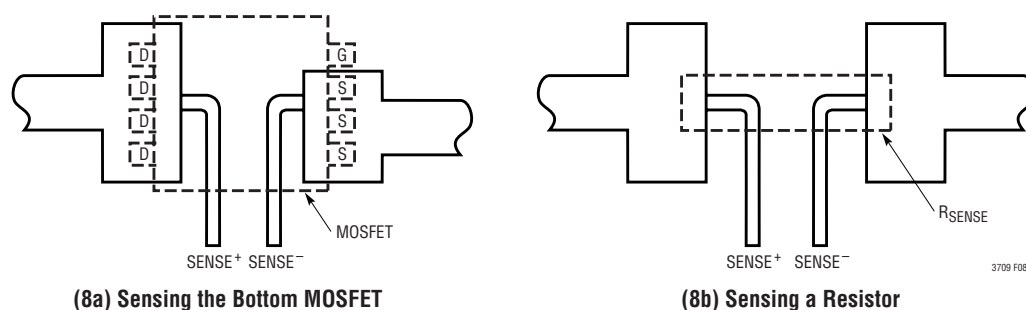
Figure 8. Kelvin Sensing
