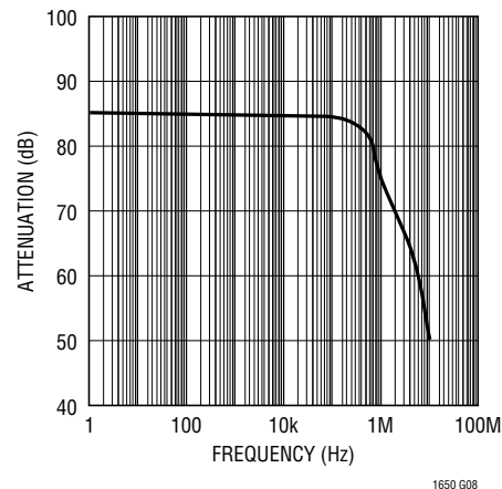
Reference Feedthrough
