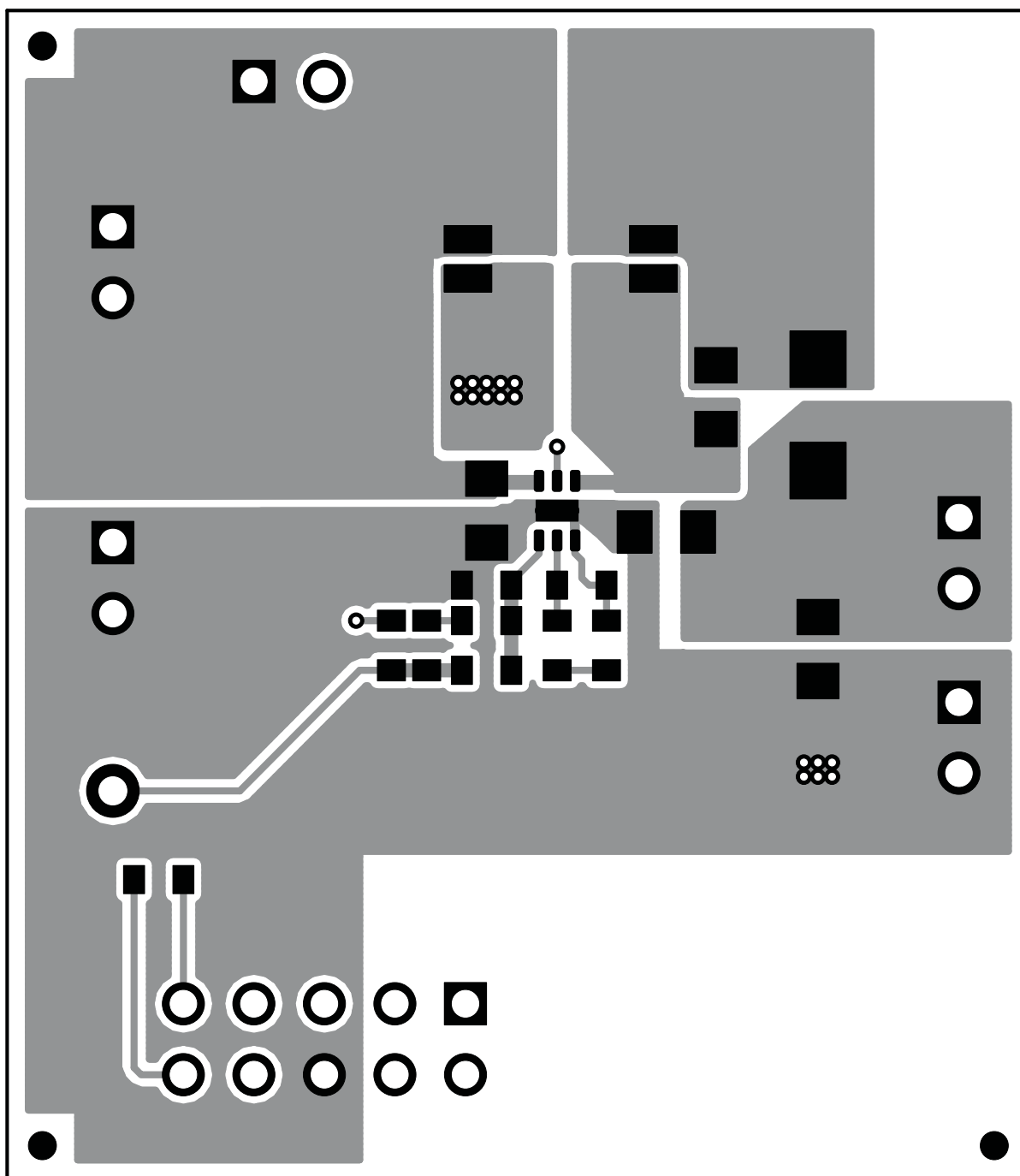
Figure 9. Top-Side Layer
