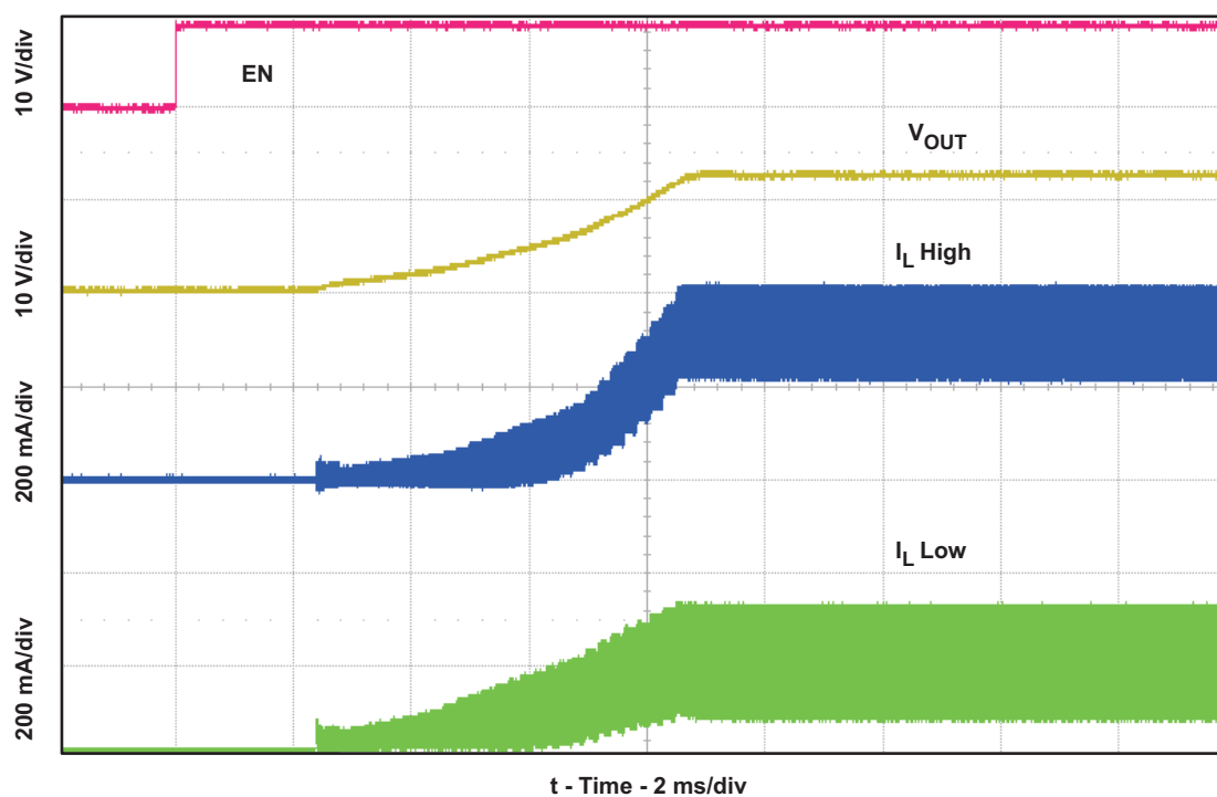
Figure 4. Start-Up With V_{IN} = 9 V and I_{OUT} = 200 mA
