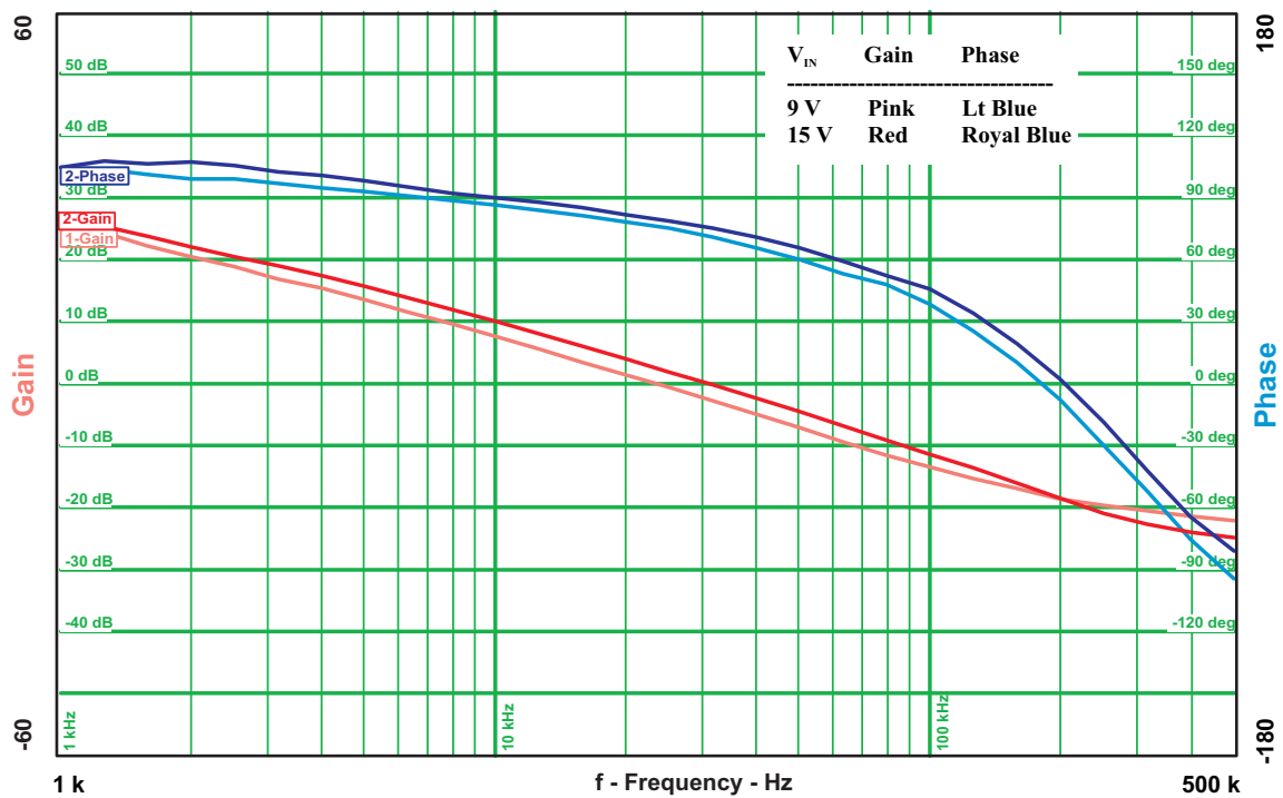
Figure 6. Loop Gain With I_{OUT} = 225 mA and V_{IN} = 9 V and 15 V
