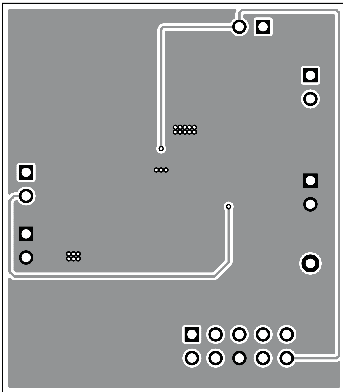
Figure 10. Bottom-Side Layer
