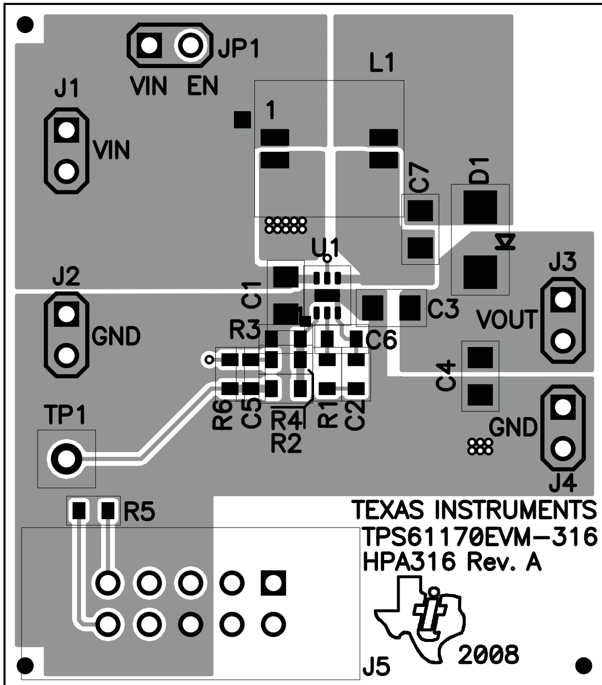
Figure 8. Top-Assembly Layer
