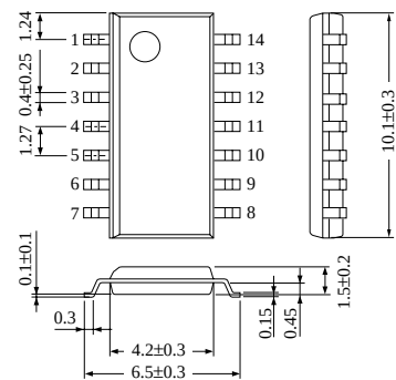
14-pin PANAFLAT Plastic Package (SOP014-P-0225A)
