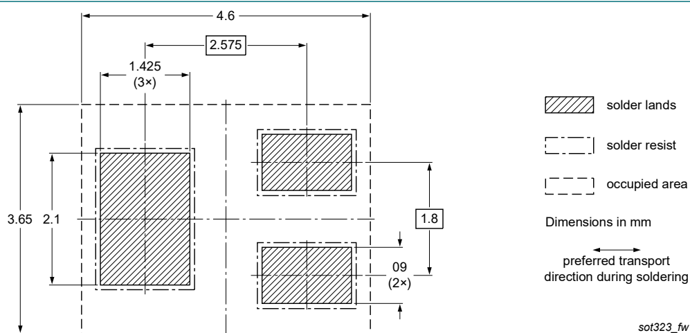
Fig. 3. Wave soldering footprint for SC-70 (SOT323)
