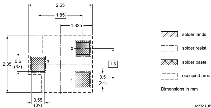
Fig. 2. Reflow soldering footprint for SC-70 (SOT323)
