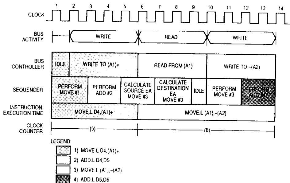
Figure 8-6. Processor Activity for Example 4
