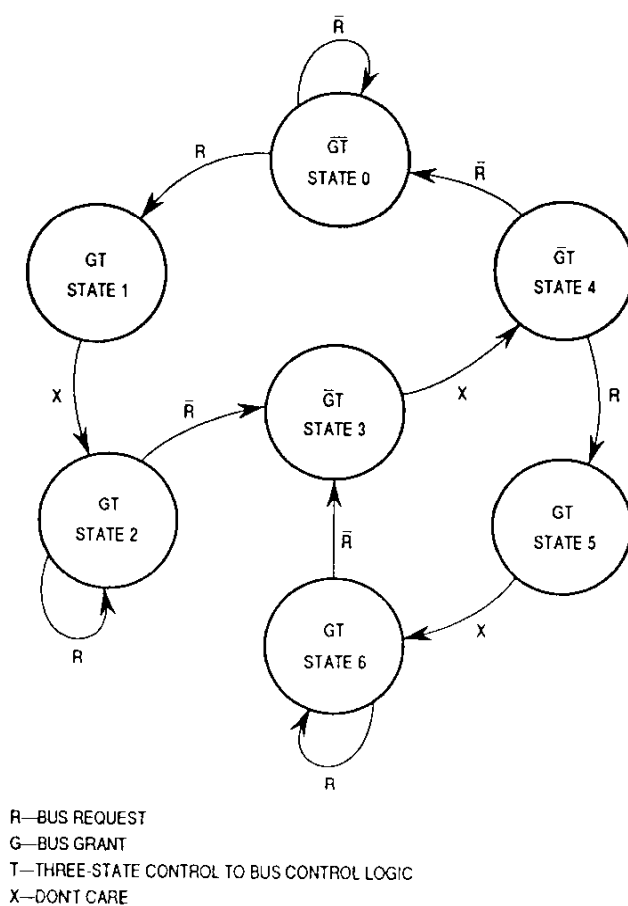
Figure 5-48. MC68EC020 Bus Arbitration State Diagram
