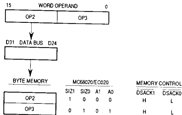
Figure 5-7. Word Operand Write to Byte Port Example
