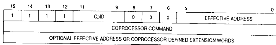
Figure 7-6. Coprocessor General Instruction Format (cpGEN)
