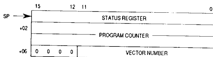
Figure 7-41. MC68020/EC020 Preinstruction Stack Frame
