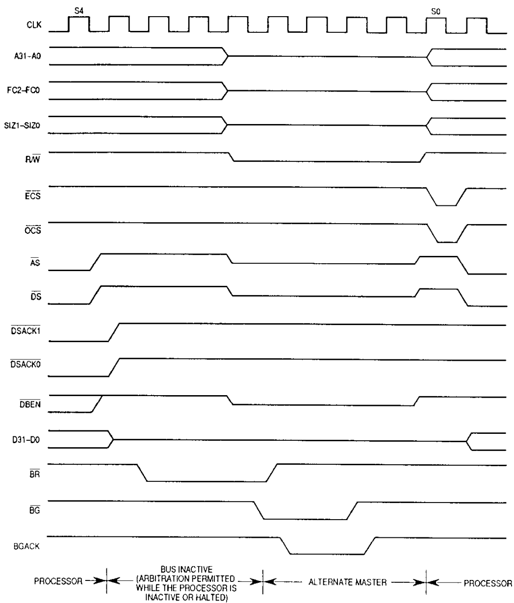
Figure 5-45. MC68020 Bus Arbitration Operation Timing—Bus Inactive
