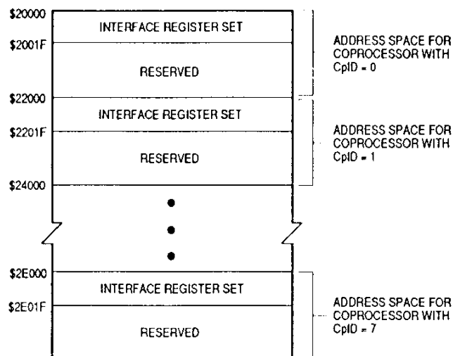
Figure 7-4. Coprocessor Address Map in MC68020/EC020 CPU Space
