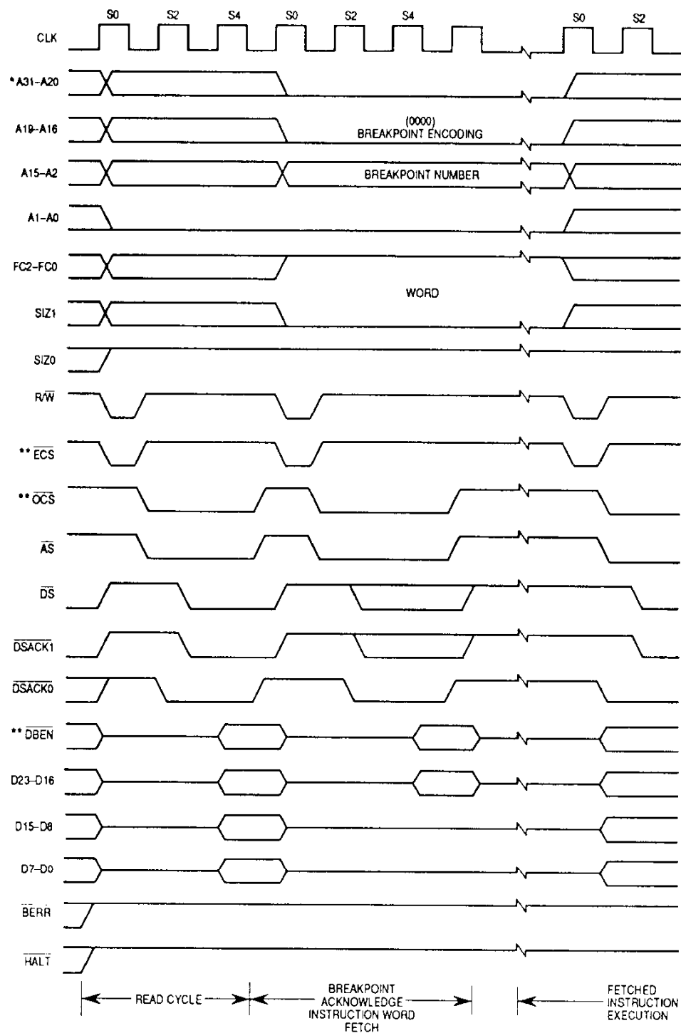
Figure 5-36. Breakpoint Acknowledge Cycle Timing
