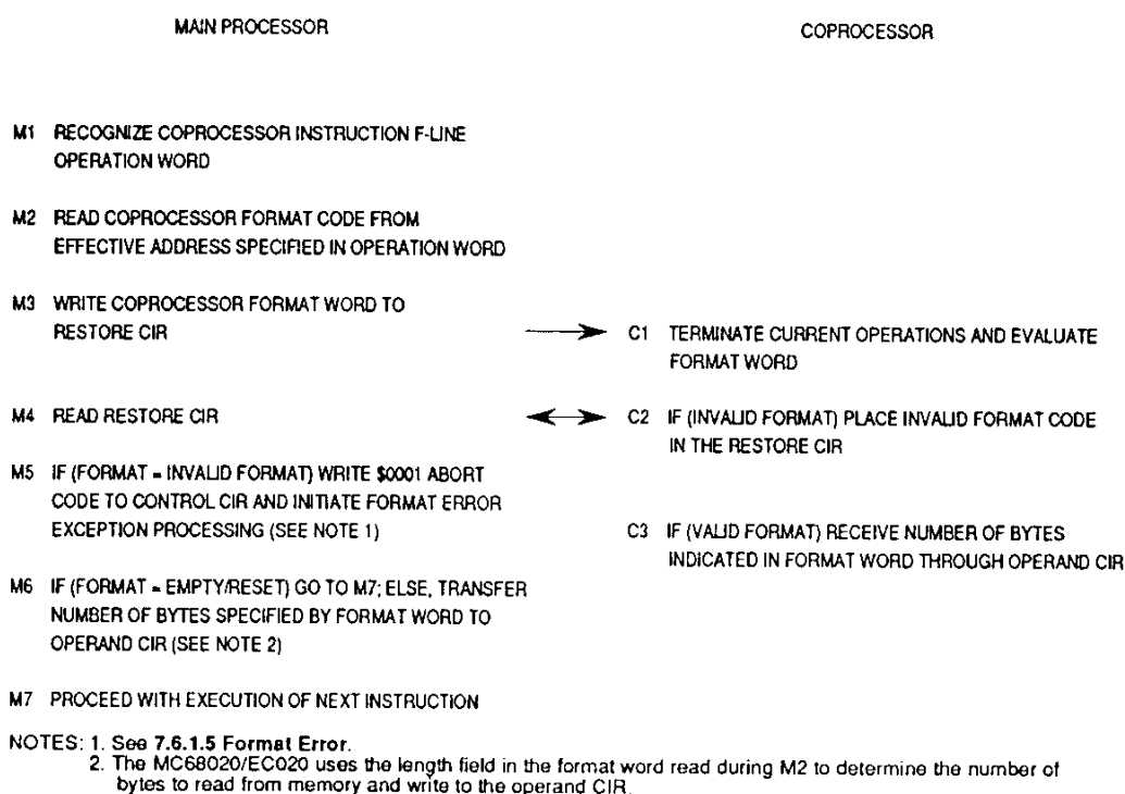
Figure 7-18. Coprocessor Context Restore Instruction Protocol
