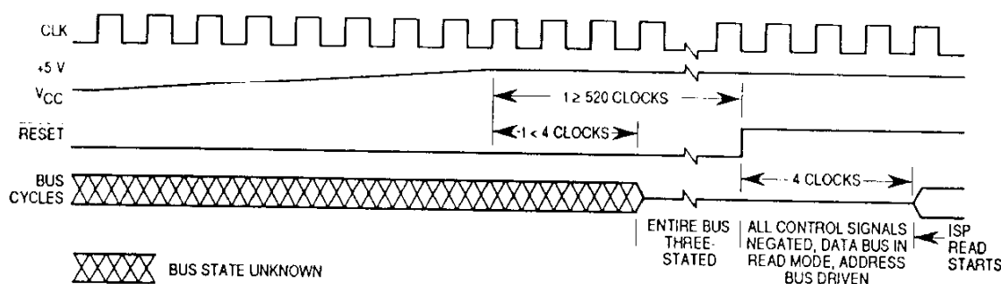
Figure 5-51. Initial Reset Operation Timing
