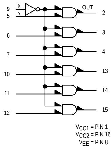
LOGIC DIAGRAM
