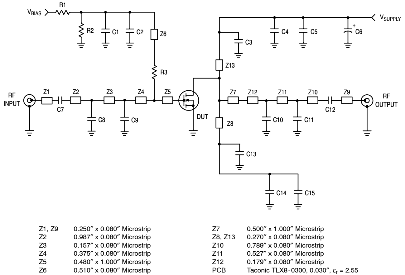
Figure 1. MRF5S21045MR1(MBR1) Test Circuit Schematic
