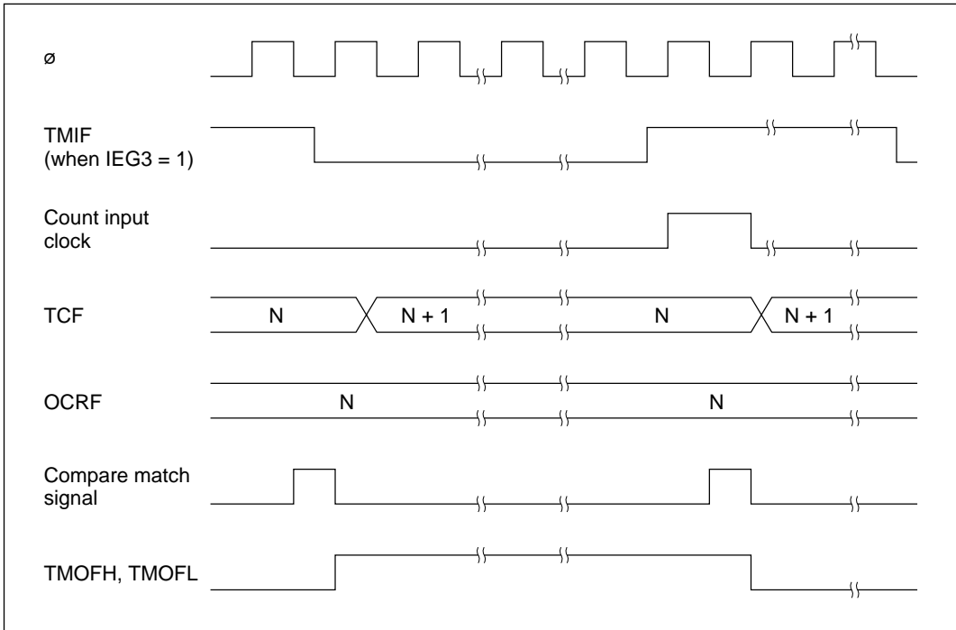
Figure 9-5 TMOFH, TMOFL Output Timing
