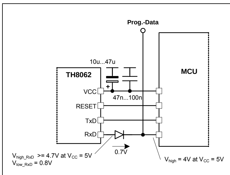
Figure 20 – Example circuitry for connection of RxD to MCU for flash programming
