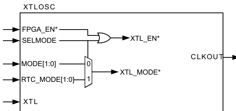
Figure 2-17 • XTLOSC Macro
