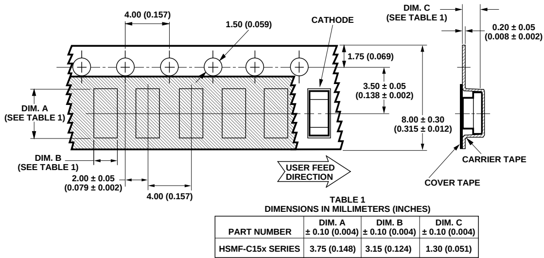
Figure 10. Tape Dimensions.
