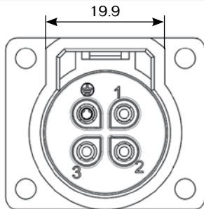
Mating face
