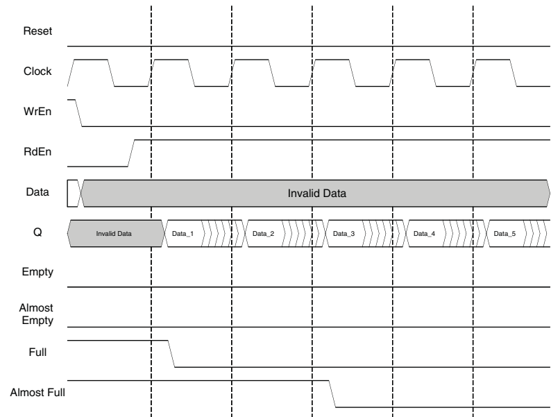
Figure 11-23. FIFO without Output Registers, Start of Data Read Cycle
