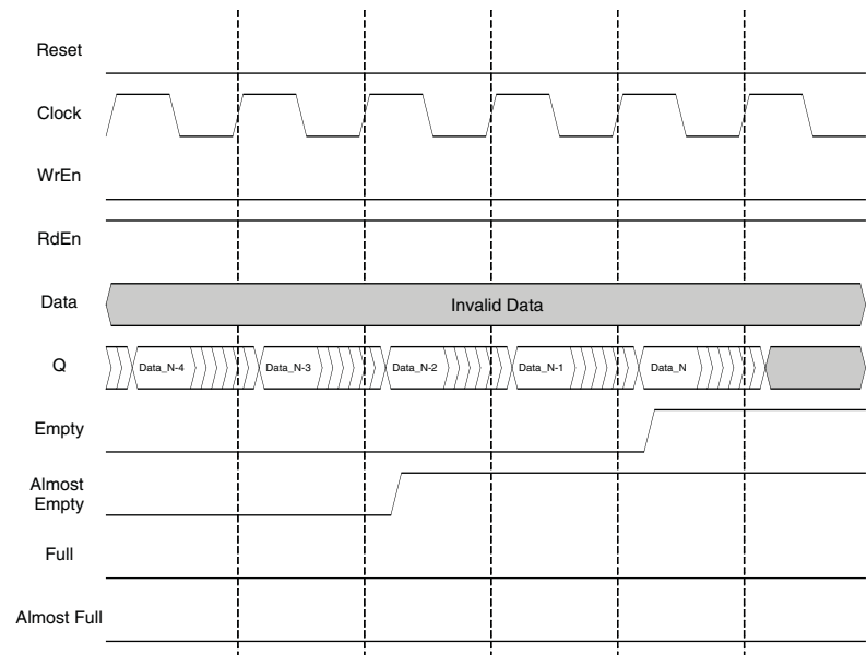
Figure 11-24. FIFO without Output Registers, End of Data Read Cycle
