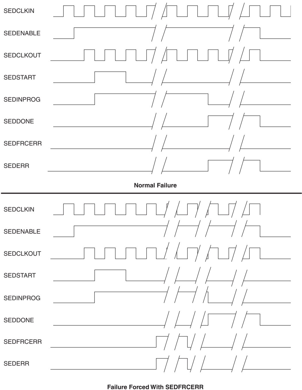
Figure 17-3. Timing Diagram
