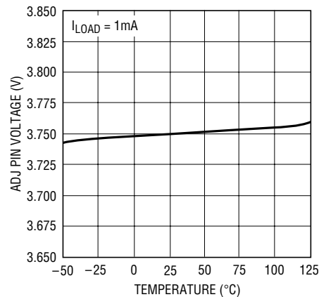
LT1529 ADJ Pin Voltage
