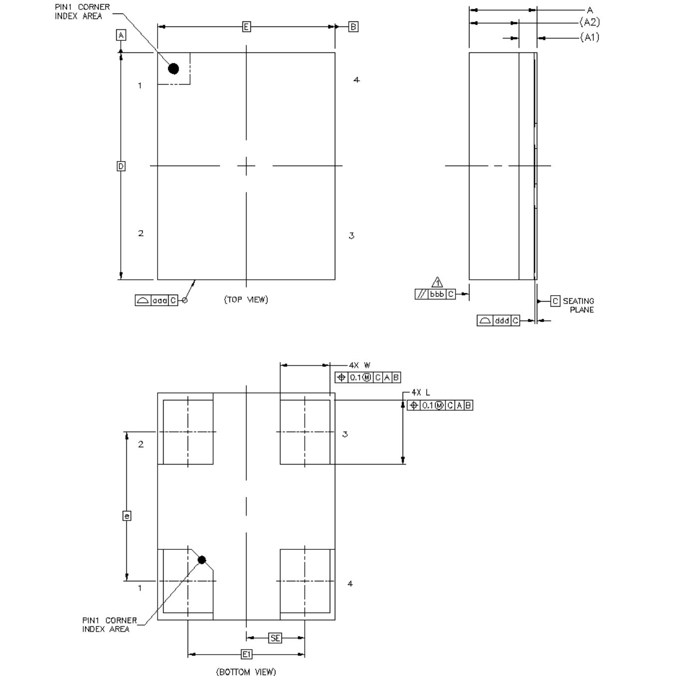
Figure 12. Si510/511 Outline Diagram
