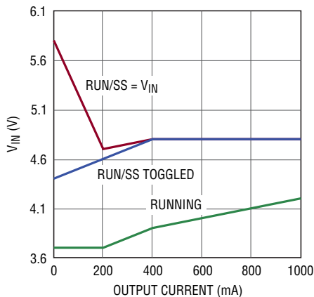
Minimum V IN vs Output Current 3.3V OUT
