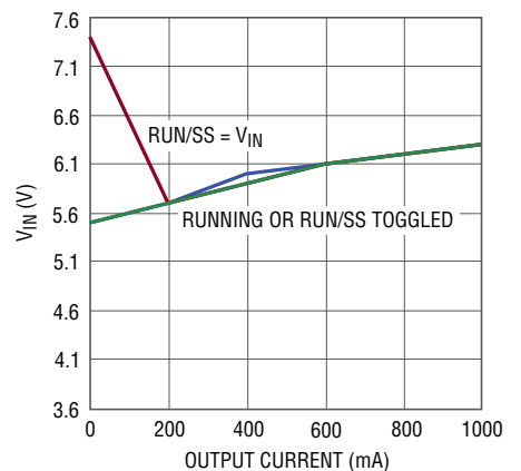
Minimum V IN vs Output Current 5V OUT
