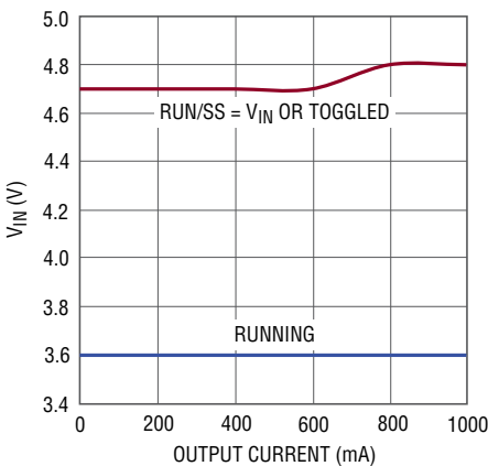
Minimum V IN vs Output Current 2.5V OUT
