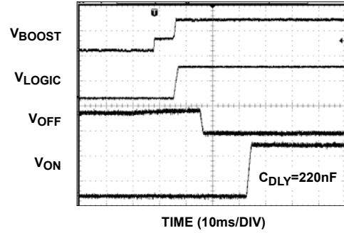
FIGURE 14. START-UP SEQUENCE
