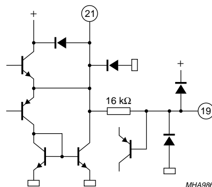
Fig.18 Pin 19; BPU and pin 21; FDI.
