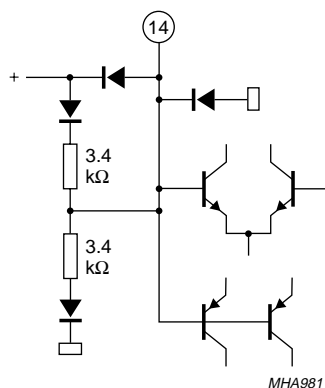
Fig.13 Pin 14; V ref .
