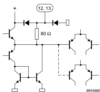
Fig.12 Pin 12; OUTL and pin 13; OUTR.
