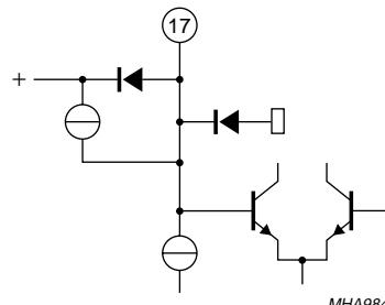
Fig.16 Pin 17; TW.
