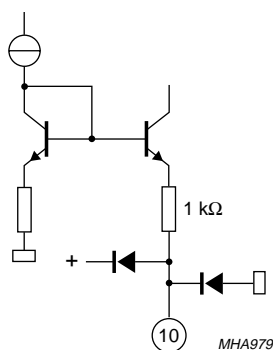
Fig.11 Pin 10; R FR .
