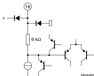
Fig.17 Pin 18; CW.
