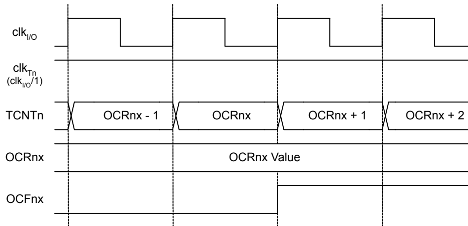
Figure 21-9. Timer/Counter Timing Diagram, Setting of OCF1x, no Prescaling
