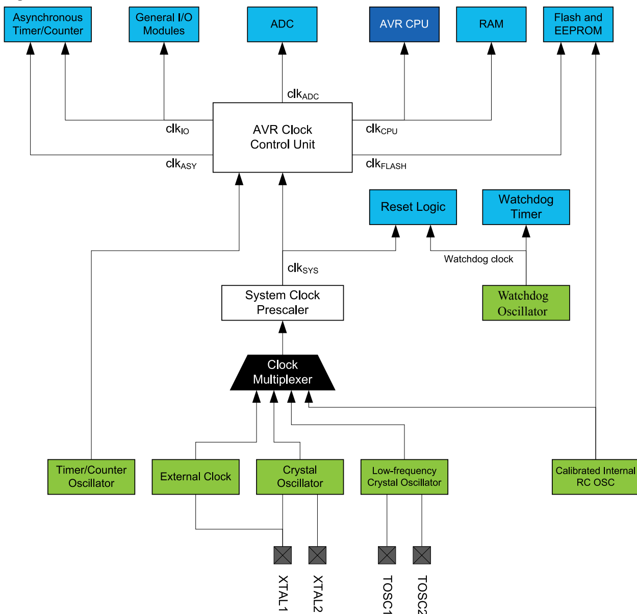
Figure 14-1. Clock Distribution
