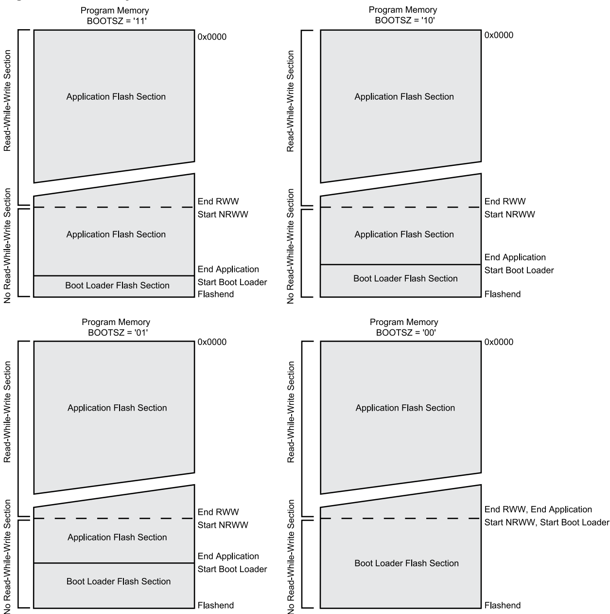
Figure 32-2. Memory Sections
