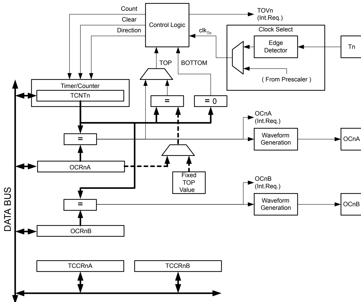
Figure 20-1. 8-bit Timer/Counter Block Diagram
