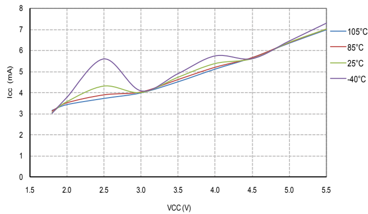
Figure 35-45. ATmega48PB_88PB: Programming Current vs. V_{CC}
