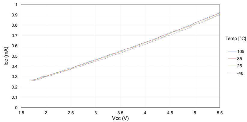
Figure 35-5. ATmega488PB/88PB: Active Supply Current vs. V_{CC} (Internal RC Oscillator, 8MHz)
