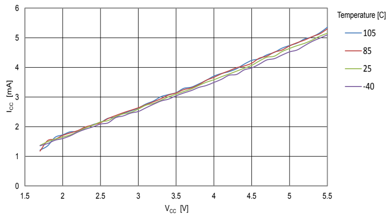
Figure 35-5. ATmega488PB/88PB: Active Supply Current vs. V_{CC} (Internal RC Oscillator, 8MHz)
