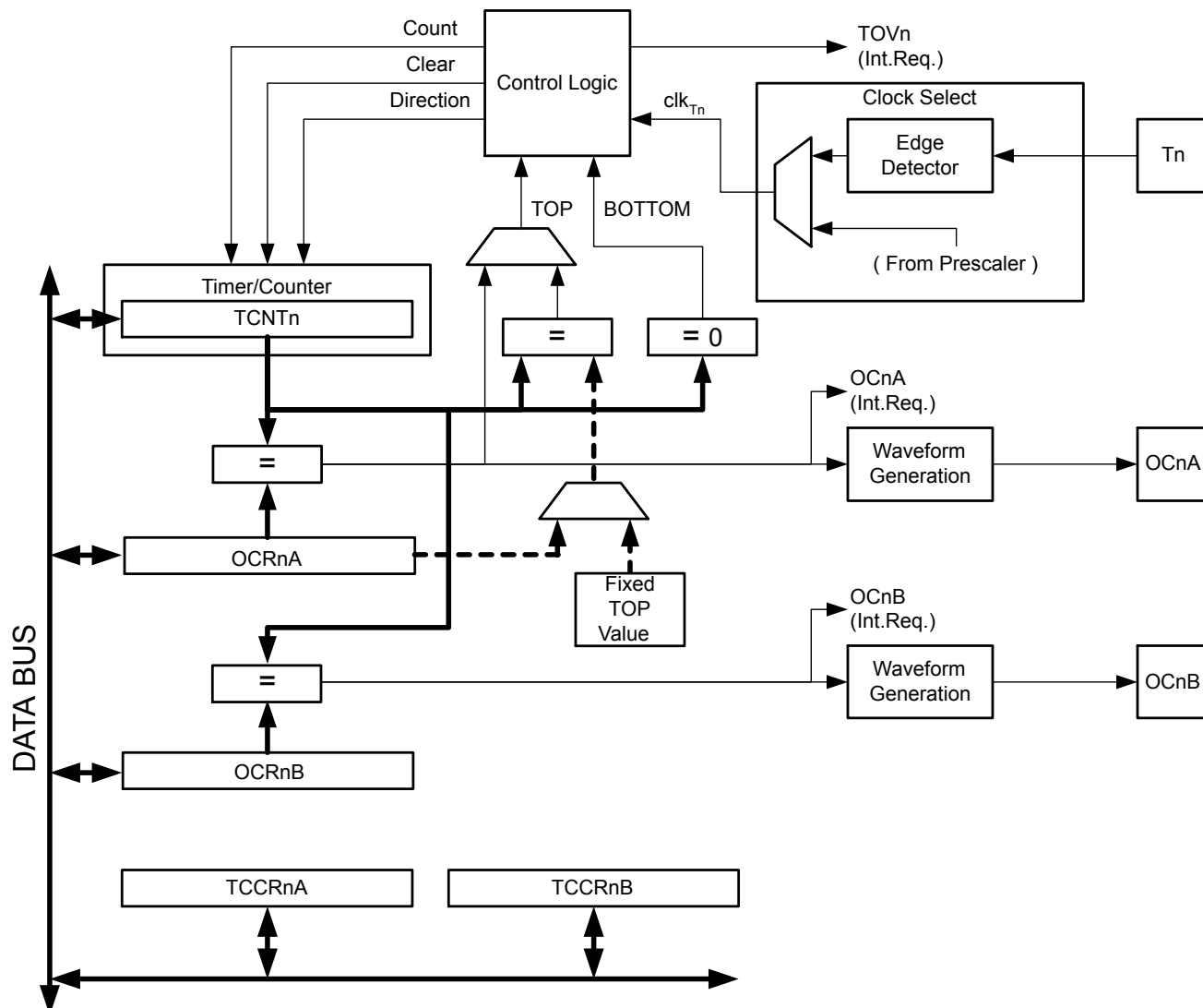
Figure 23-1. 8-bit Timer/Counter Block Diagram
