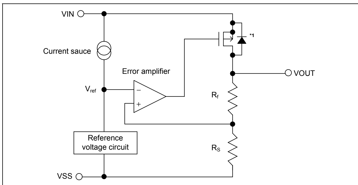
Figure 11 Block diagram
