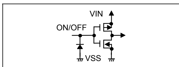
Figure 12 The structure of the ON/OFF Pin
