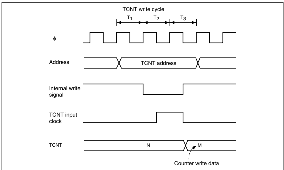
Figure 11.8 Contention between TCNT Write and Increment
