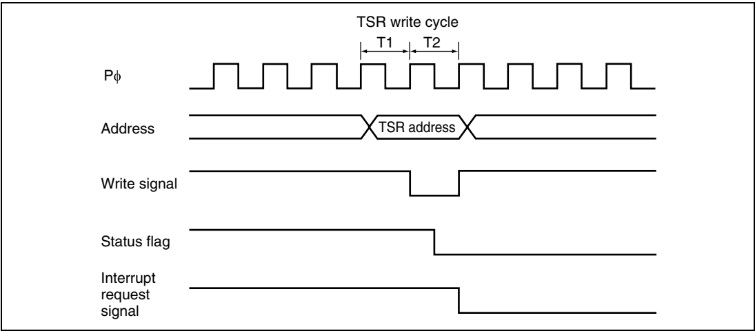
Figure 15.13 Timing of Status Flag Clearing by CPU
