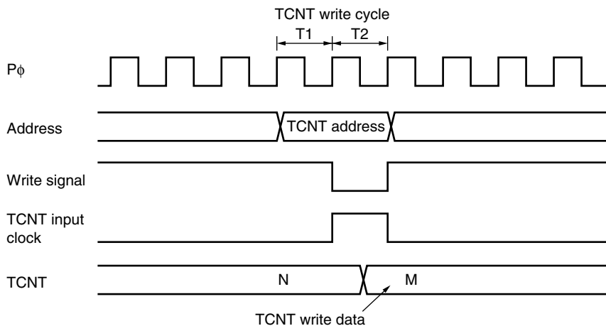
Figure 10.72 Contention between TCNT Write and Increment Operations
