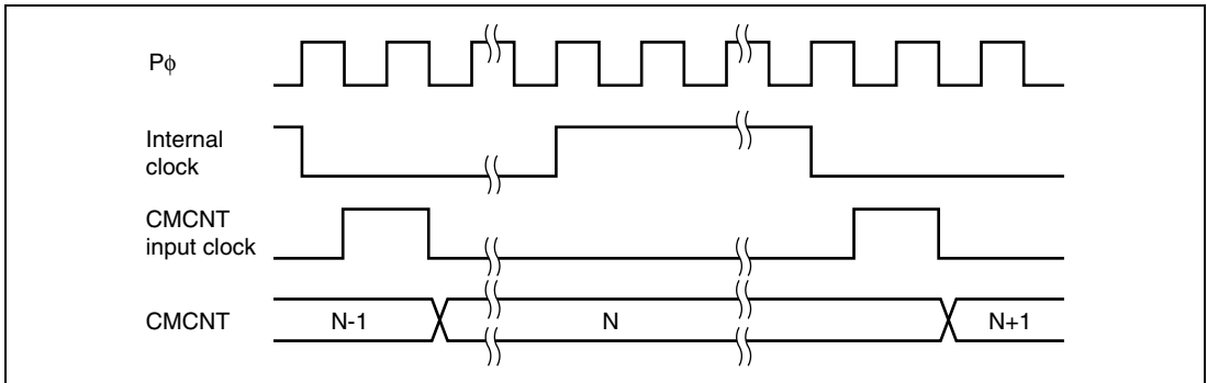
Figure 14.3 Count Timing
