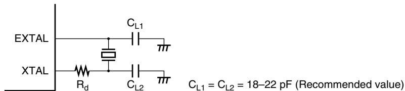
Figure 4.2 Connection of the Crystal Resonator (Example)
