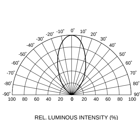
Fig. 3 Radiation Diagram
