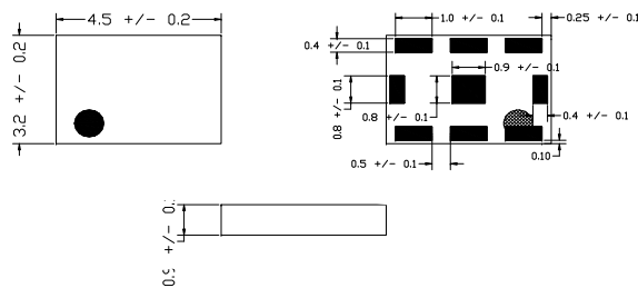
[MECHANICAL DIMENSIONS]
