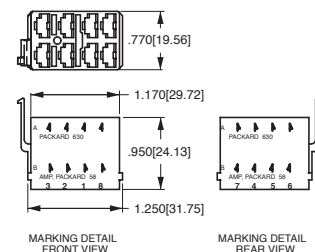
VCH CONNECTOR HOUSING
