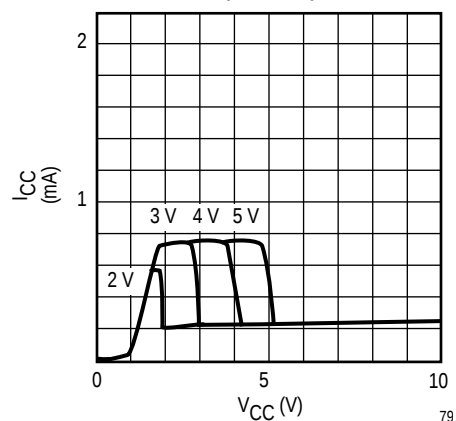
SUPPLY VOLTAGE vs. INPUT CURRENT (NO LOAD)
