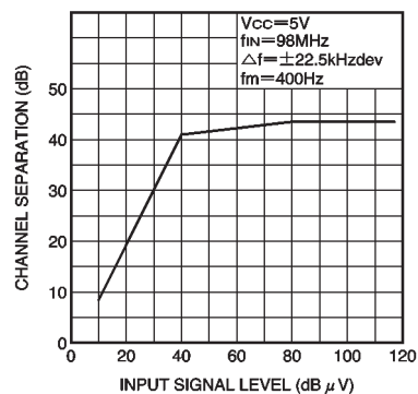
Fig. 28 Sensitivity characteristics
