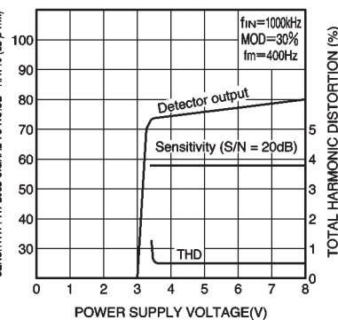
Fig. 22 Power supply voltage characteristics
