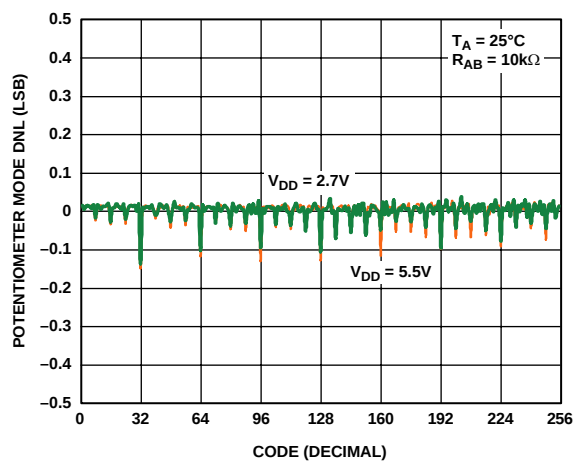
Figure 8. DNL vs. Code vs. Supply Voltages
