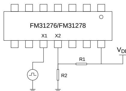
Figure 10. External Oscillator
