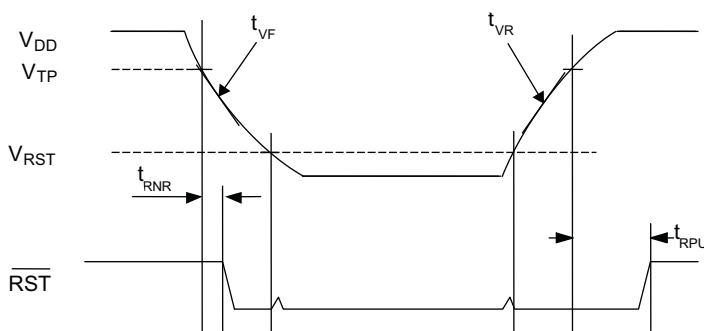
Figure 24. \overline{RST} Timing
