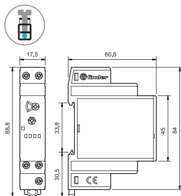
80.21 Screw terminal
