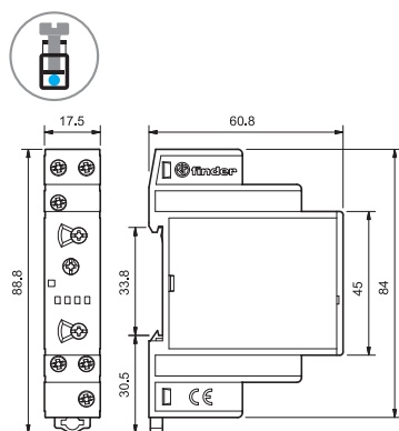
80.01 Screw terminal
