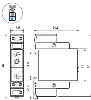
80.82 Screw terminal
