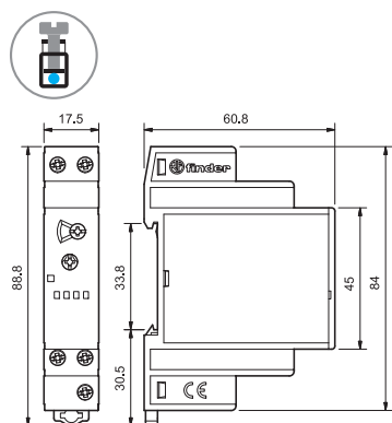
80.61 Screw terminal
