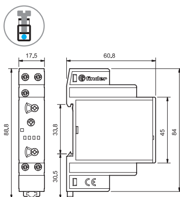
80.71 Screw terminal
