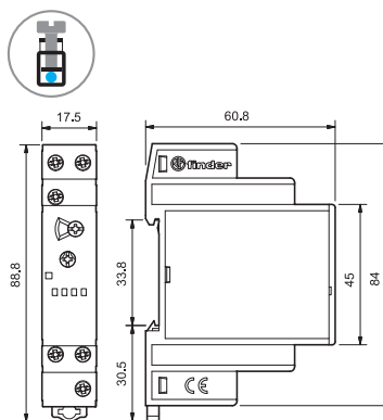
80.41 Screw terminal
