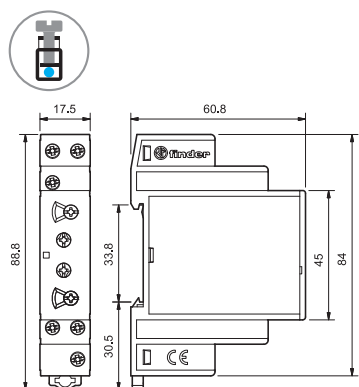
80.91 Screw terminal
