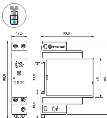
80.11 Screw terminal
