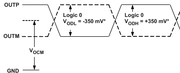
Figure 2. LVDS Output Voltage Levels
