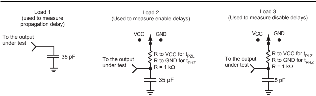
Figure 1-15 • AC Test Loads
