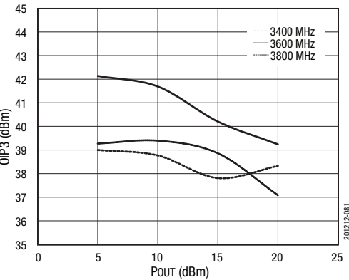
Figure 81. OIP3 vs Pout
