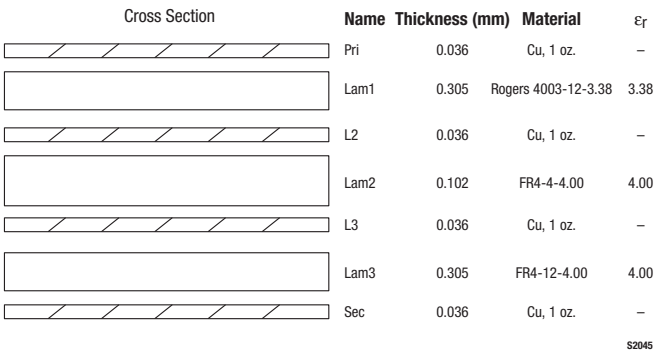
Figure 85. Layer Detail Physical Characteristics
