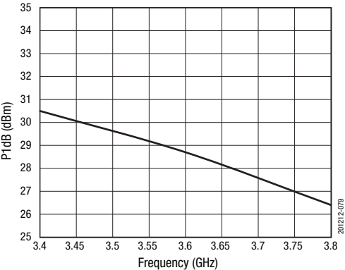
Figure 79. P1dB vs Frequency
