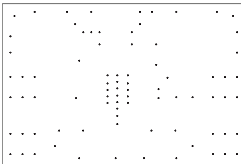
Layer 3: Ground
