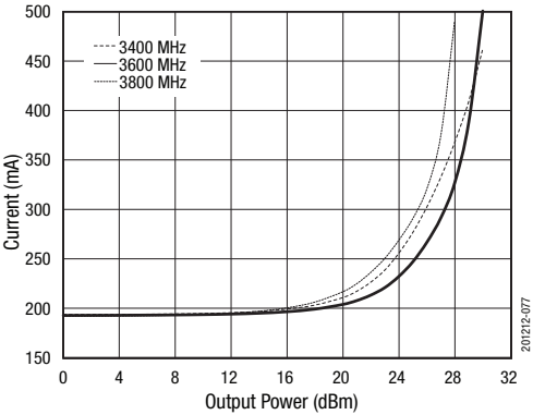
Figure 77. Current vs Output Power
