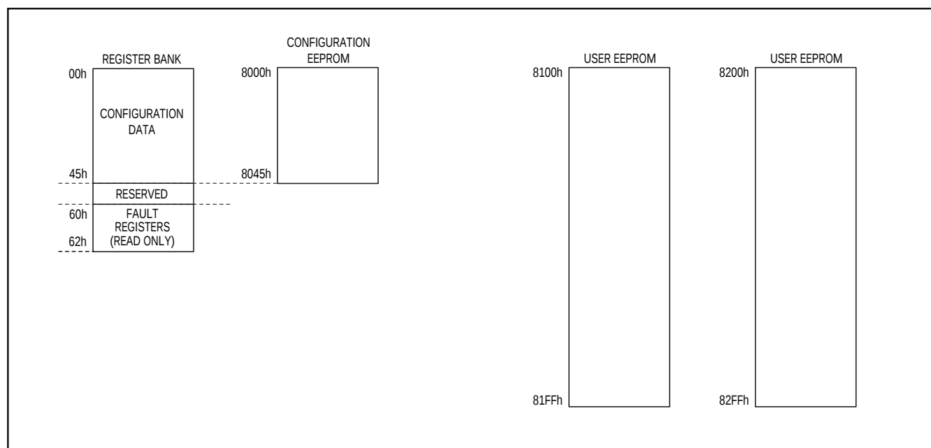
Figure 8. Memory Map
