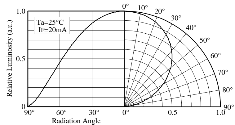
■ Directivity (NSCB455A)
