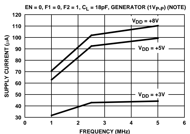
FIGURE 16. DISABLED SUPPLY CURRENT vs FREQUENCY
